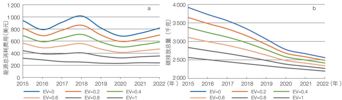
图3 2015—2022年道路汽车单车年度能源总消耗费用（a）与总碳排放量（b）情景分析 Figure 3 Scenario analysis of road vehicle energy consumption (a) and carbon emissions (b) per single electric vehicle from 2015 to 2022
