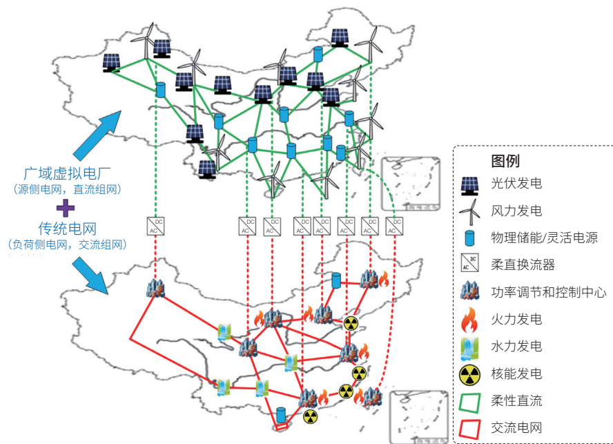
图2 广域虚拟电厂（源侧电网）与传统电网（负荷侧电网）叠加构建新型电力系统 Figure 2 Future power system based on traditional power system (load side grid) and wide-area virtual power plant (power-source side grid)
